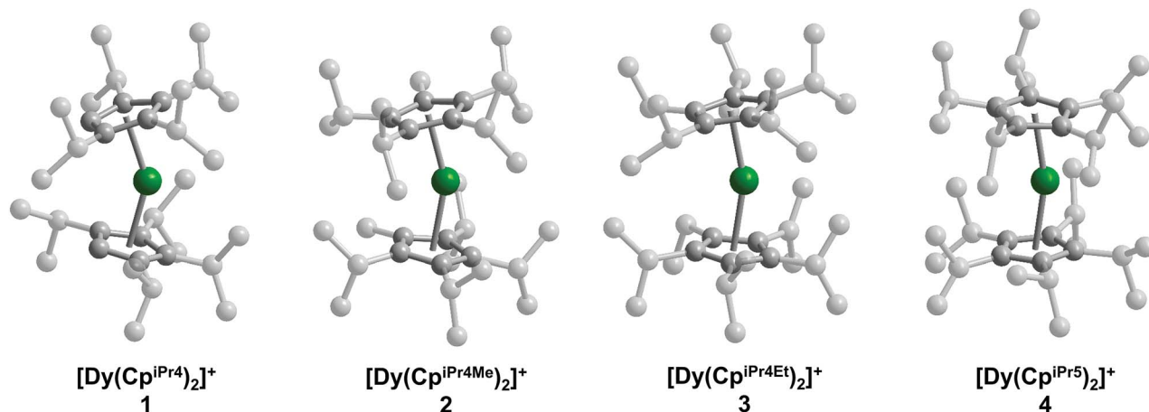
Fig. 1 Structures of the metallocenium complexes in crystals of [\text{Dy}(\text{Cp}^{\text{iPr}^{\text{R}}})_2][\text{B}(\text{C}_6\text{F}_5)_4] ( \text{R} = \text{H} (1), Me (2), Et (3), iPr (4)). Green and gray spheres represent Dy and C atoms, respectively; hydrogen atoms, [\text{B}(\text{C}_6\text{F}_5)_4]^- counteranions, and positional disorder are omitted for clarity.
