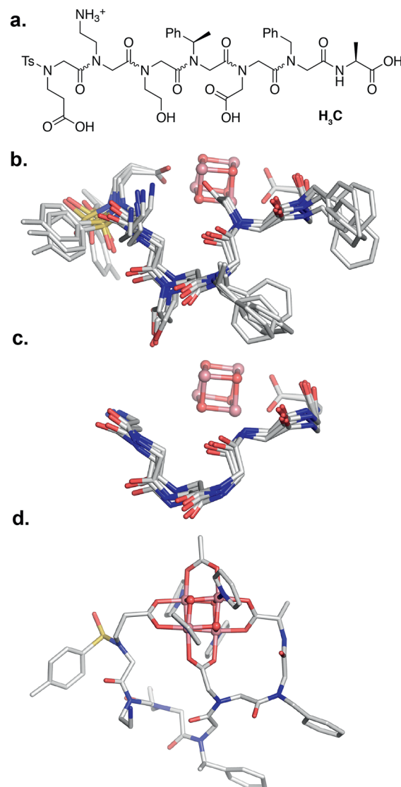
Fig. 4 (a) Primary sequence of peptoid H 3 C. (b) Overlay of the five lowest energy NMR structures, with pyridine and acetate removed for clarity. (c) Peptoid backbone view only. (d) A selected low energy NMR structure.
