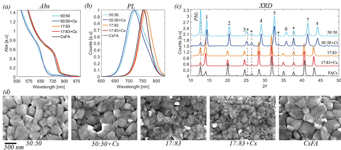
Fig. 1 (a) UV-vis absorption for the five compositions investigated. Data is corrected for the background. Raw data is available in the ESI.† (b) Steady state photoluminescence. Normalised data. (c) X-ray diffraction data for perovskite films deposited on FTO/TiO 2 substrates. The labelled peaks correspond to: 1 [001], 2 [011], 3 [111], 4 [002], 5 [012, 102], 6 [112], 7 [022], 8 [003, 112]. Peaks originating from the substrate are marked by * (d) top view SEM images for the five different compositions. Images at different resolution are available in the ESI.†
