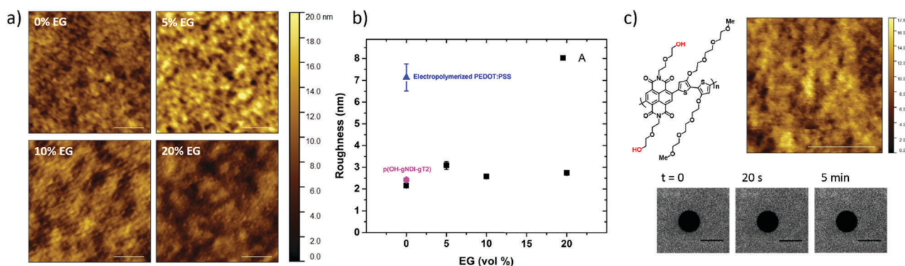
Fig. 4 (a) AFM topography images of the PEDOT:PSS films in PBS at pH 7.4. The films were cast from dispersions with various EG concentrations and the images were taken after DI water immersion and \text{O}_2 plasma activation. Scale bar = 500 nm; (b) surface roughnesses of the hydrated films with various EG contents (A: black squares) and those of the electropolymerized PEDOT:PSS (blue triangle) and p(OH-gNDI-gT2) (pink hexagon) after treatment and (c) AFM topography image of the p(OH-gNDI-gT2) film in PBS at pH 7.4 after water immersion and \text{O}_2 plasma activation. The FRAP images show no recovery of fluorescence when lipids were deposited on such a polymer surface. The scale bars for the AFM and FRAP images are 400 nm and 20 \mu\text{m} , respectively.
