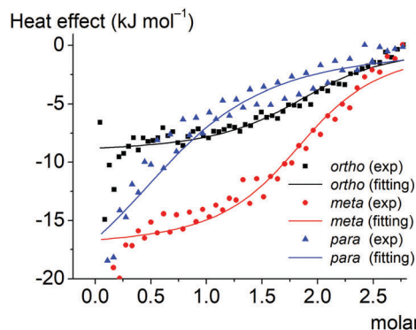
Fig. 8 The experimental (depicted in the points) and fitted (depicted in the solid lines) plots of the binding heat effect versus the BSA-to-clathrochelate molar ratio for the ortho -, meta - and para -substituted hexacarboxyphenyl-terminated iron(II) clathrochelates 1–3 as guests.
