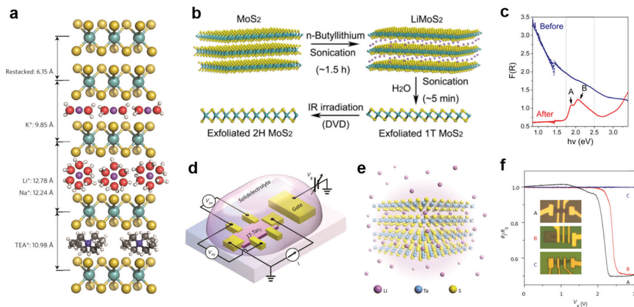
Fig. 9 Intercalation modulation of MXs: (a) intercalation of MoS 2 by alkali ions ( Li^+ , Na^+ , K^+ ) with solvent molecules, and by TEA^+ , reprinted with permission from ref. 193, Copyright 2015 Nature Publishing group. (b) Sonication assisted exfoliation of MoS 2 in the 1T phase and IR irradiation assisted restoration; (c) the resulting reflectance spectral change, reprinted with permission from ref. 200, Copyright 2015 American Chemical Society. (d) The electrochemical setup and (e) the illustration of Li intercalation in TaS 2 ; (f) patterned control of Li^+ intercalation into devices and the resulting gate modulation characteristics, reprinted with permission from ref. 40, Copyright 2015 Nature Publishing group.
