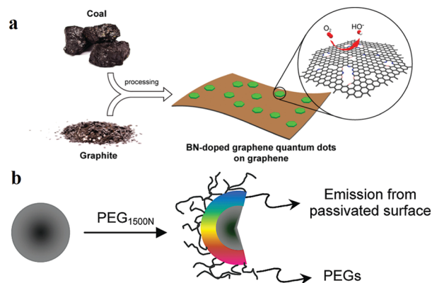
Fig. 3 Schematic representations of the heteroatom doping and surface passivation approaches of CD functionalisation, reprinted with permission from ref. (a) Illustration of the preparation procedure for the BN-GQD/graphene nanocomposite, reprinted with permission from ref. 93, Copyright 2014, American Chemical Society. (b) Functionalisation of CD surfaces with PEG, reprinted with permission from ref. 14, Copyright 2006, American Chemical Society.
