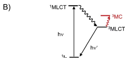
Fig. 1 Photoinitiated ligand exchange in ruthenium polypyridyl complexes. (A) Photolysis observed for Ru(II)-nitrile complexes is a two-step process in which both ligands are exchanged with coordinating solvent. (B) Jablonski diagram showing excited states responsible for ligand.
