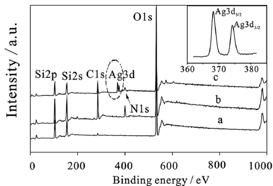
Fig. 14 XPS spectra of (a) m\text{SiO}_2 , (b) m\text{SiO}_2@NH_2 and (c) m\text{SiO}_2@NH_2@Ag ; inset is the high resolution Ag 3d XPS spectra of m\text{SiO}_2@NH_2@Ag 41 (adapted with permission from Royal Society of Chemistry, 2015).
