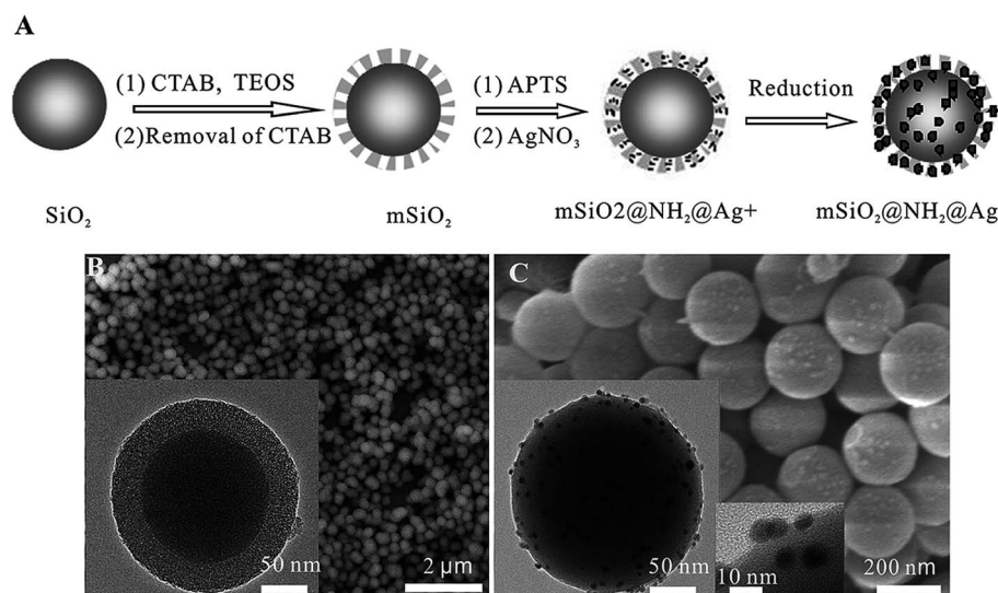
Fig. 13 (A) Schematic illustration of the procedure for the preparation of m\text{SiO}_2@NH_2@Ag . (B) SEM image of m\text{SiO}_2 microspheres. (C) SEM image of m\text{SiO}_2@NH_2@Ag . The insets show the low-magnification and high-magnification TEM images of m\text{SiO}_2@NH_2@Ag 41 (adapted with permission from Royal Society of Chemistry, 2015).
