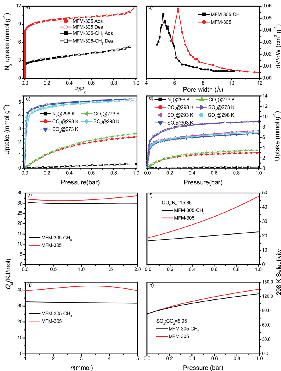
Fig. 2 Gas adsorption data. (a) Adsorption isotherms for N 2 in MFM-305-CH 3 and MFM-305 at 77 K and 1.0 bar. (b) Comparison of the pore size of MFM-305-CH 3 and MFM-305. (c) Adsorption isotherms for CO 2 , SO 2 and N 2 in MFM-305-CH 3 at 273 and 298 K and 1.0 bar. (d) Adsorption isotherms for CO 2 , SO 2 and N 2 in MFM-305 at 273, 293, 298 and 303 K and 1.0 bar. Variation of isosteric heat of adsorption Q st as a function of (e) CO 2 and (g) SO 2 uptake for MFM-305-CH 3 and MFM-305 calculated from adsorption isotherms measured at 273 and 298 K. Comparison of the IAST selectivity of (f) CO 2 /N 2 (15 : 85) and (h) SO 2 /CO 2 (5 : 95) in MFM-305-CH 3 and MFM-305 at 298 K.
