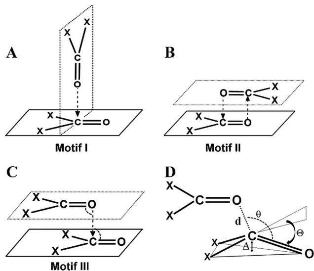
Fig. 1 Different structural motifs previously observed by Allen et al. in intermolecular \text{CO}\cdots\text{CO} interactions in ketone dimers (A) perpendicular motif I, (B) antiparallel motif II, (C) sheared parallel motif III and (D) various structural parameters that are indicative of n \rightarrow \pi^* interactions.
