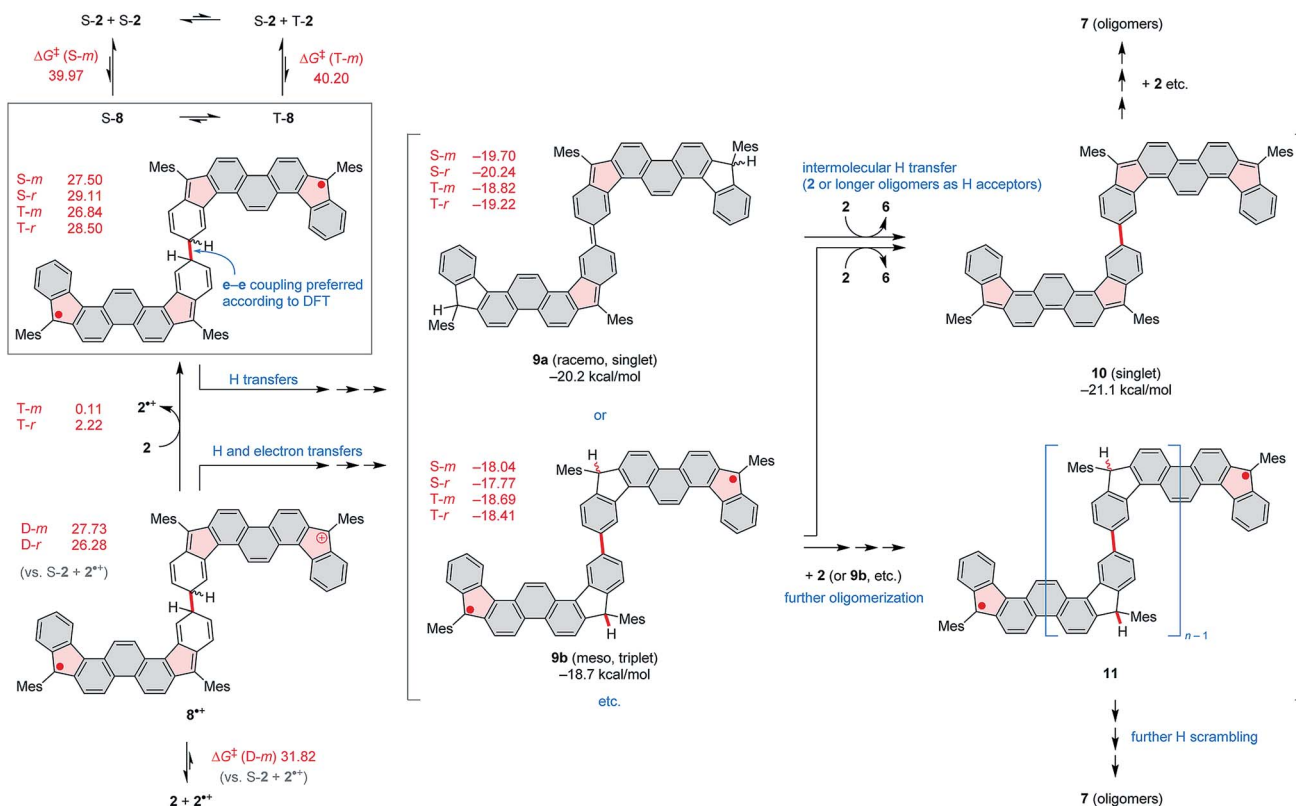
Scheme 5 Potential oligomerization pathways for 2 . Gibbs free energies (red labels, kcal mol -1 , UCAM-B3LYP/6-31G(d,p), gas phase, 298 K) are given relative to S-2 + S-2, unless indicated otherwise. S, D, and T indicate respectively the broken-symmetry-singlet, doublet and triplet wavefunctions. r and m indicate the racemic pair and the meso isomer, respectively.
