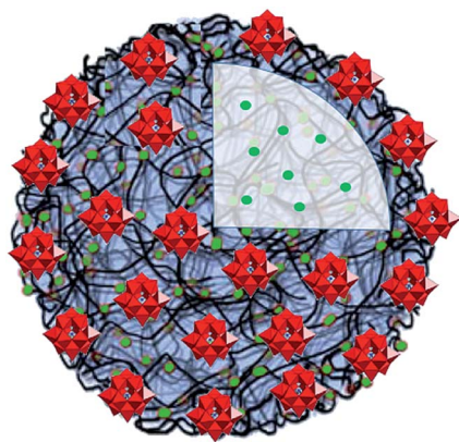
Fig. 10 The POM coacervate vesicle formed by the Keggin-type [\text{PW}_{11}\text{O}_{39}]^{7-} units, ATP (green spheres) and PDDA (black bent lines). Colour code: W, red polyhedra; P, blue spheres. Adapted with permission from ref. 65. Copyright 2014 of Wiley-VCH Verlag GmbH & Co. KGaA.
