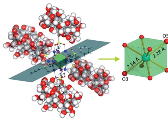
Fig. 11 Representation of the fragment of the solid-state structure of \text{K}_6[\{\text{CoO}_8\text{Pd}_{12}(\text{C}_6\text{H}_5\text{AsO}_3)_8\} \subset 2\{\text{C}_{36}\text{H}_{60}\text{O}_{30}\}] \cdot 25\text{H}_2\text{O} \cdot \text{KCl} , emphasizing the elongation of the \{\text{CoO}_8\} unit (transparent green) along one of its diagonal planes. Bonds in the two \alpha -CD-incorporated phenyl-arsonates are shown in black. Counterions, water and co-crystallised KCl molecules are omitted for clarity. Color code: Co, turquoise; Pd, blue; As, yellow; O, red; C, black/grey; H, white spheres. Reprinted with permission from ref. 74c. Copyright 2018 of Wiley-VCH Verlag GmbH & Co. KGaA.
