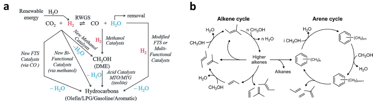
Fig. 7 (a) Schematic illustration of \text{CO}_2 hydrogenation to \text{C}_{2+} products via the \text{CO} intermediate route and \text{CH}_3\text{OH} intermediate route. Reprinted from ref. 12 with permission from the Royal Society of Chemistry. (b) General scheme of the dual-cycle mechanism during the MTH process. Reprinted from ref. 44 with permission from Elsevier.
