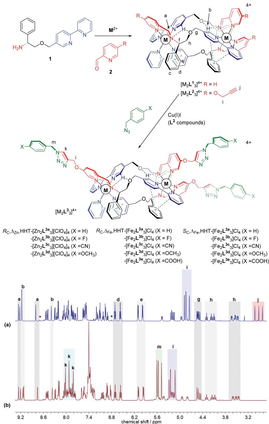
Fig. 1 Metallohelix architectures via asymmetric self-assembly and CuAAC. Synthesis of the new alkyne-appended triplex enantiomers [M_2L^3_3]^{4+} gives access to a range of optically pure structures of Zn(II) and Fe(II); the stereochemical descriptors for the complexes e.g. R_C, \Delta, HHT refer to the absolute configurations at C, the metal, and the directionality of the ligand strands respectively. ^1H NMR spectra (500 MHz, CD_3CN , 298 K) show clean conversion of (a) R_C-\Delta_{Zn}-HHT-[Zn_2L^3_3][ClO_4]_4 to (b) R_C-\Delta_{Zn}-HHT-[Fe_2L^3_3][ClO_4]_4 . Alkyne resonances j are replaced by triazole singlets k but otherwise the triplex architecture is unperturbed; * indicates resonances assigned to the HHH isomer.
