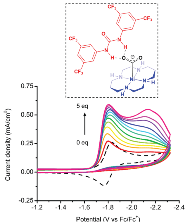
Fig. 14 Cyclic voltammograms showing [\text{Ni}(\text{cyclam})]^{2+} (40, 1 mM) under Ar (black dashed line) and under \text{CO}_2 (colored lines) with 0–5 equivalents of bis(3,5-trifluoromethyl)-phenylurea (Schreiner's urea, see the inset) as an additive. Reprinted with permission from ref. 230. Copyright 2019 American Chemical Society.
