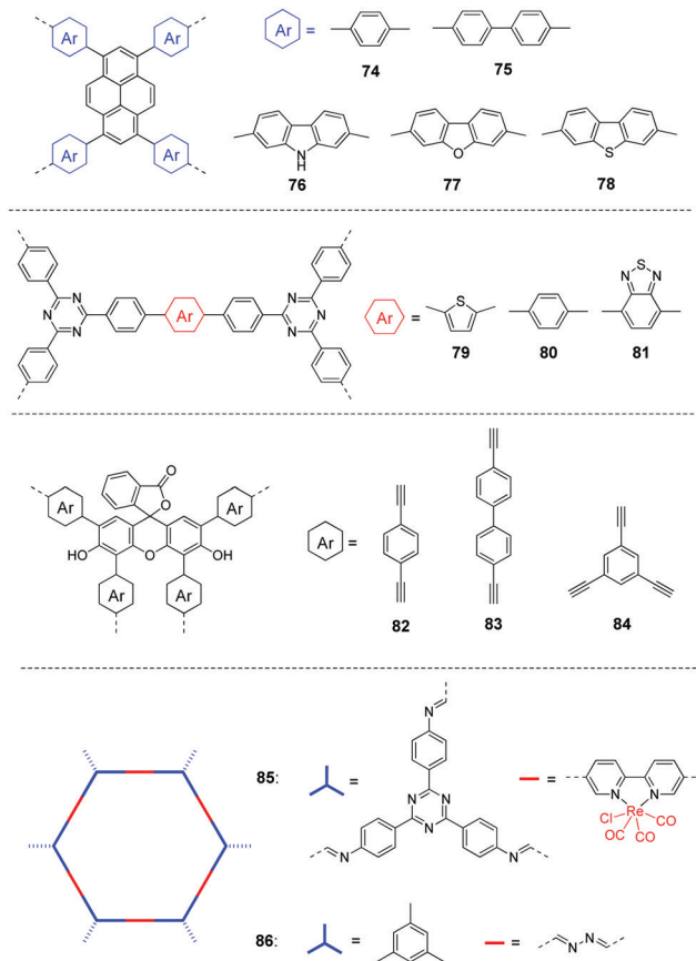
Fig. 18 Chemical structures of polymers 74–86 for photocatalytic CO 2 reduction.
