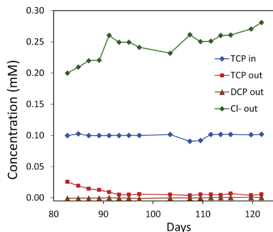
Fig. 6 Degradation of TCP by a mixed culture of P. putida strains MC4-5221, MC4-1331 and A. radiobacter AD1 in a laboratory-scale aerated packed bed bioreactor operated in a continuous mode. Packing material was sintered glass and data were collected after an initial 80 day acclimation period. TCP loading rate 0.40–0.44 mg h -1 l -1 ; residence time 23 h; removal increasing to 95%. 40,62
