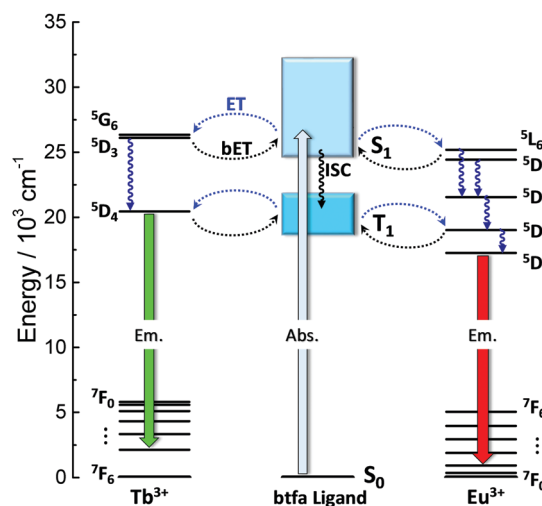
Fig. 7 Schematic partial energy level diagram of the [C_4mim][Tb_{1-x}Eu_x(btfa)_4] ( x = 0.01, 0.05 and 0.10 ) complexes involving the btfa ligand, Eu^{3+} and Tb^{3+} electronic states. T_1 is the lowest ligand triplet level and S_0 and S_1 are the ligand ground and lowest singlet excited states, respectively. Abs. is the initial absorption, ISC is the intersystem crossing and Em is the emission. ET and bET are the forward and backward energy transfer, respectively.
