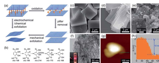
Fig. 4 (a) Illustration of the synthetic process of 2D MOFs by using the electrochemical/chemical exfoliation method and (b) a possible oxidative transformation route from H_4d\text{hdbc} to a species with m/z 168. SEM images of (c) 3D-Co, (d) 2D-Co, and (e) 2D-Co-NS. (f) TEM image of 2D-Co-NS (inset: Tyndall effect of a colloidal solution). (g) AFM image and (h) the corresponding height profile of 2D-Co-NS. Reproduced with permission. 77 Copyright©2018 WILEY-VCH Verlag GmbH & Co. KGaA.
