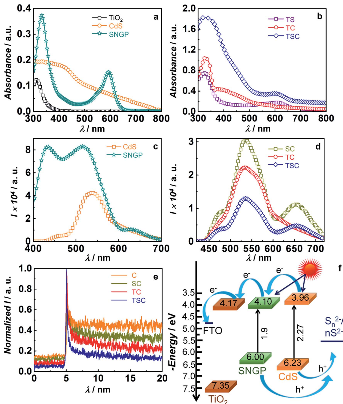
Fig. 3 Absorbance spectra of (a) \text{TiO}_2 , CdS and SNGPs and (b) \text{TiO}_2/\text{SNGP} (TS), \text{TiO}_2/\text{CdS} (TC) and \text{TiO}_2/\text{SNGP}/\text{CdS} (TSC). Fluorescence spectra of (c) CdS (C), SNGPs and (d) SNGP/CdS (SC), \text{TiO}_2/\text{CdS} , and \text{TiO}_2/\text{SNGP}/\text{CdS} composites recorded at \lambda_{\text{ex}} of 370 nm. (e) Emission decay plots for photoactive electrodes measured at an \lambda_{\text{ex}} of 370 nm and at an \lambda_{\text{em}} of 534 nm. (f) Energy level diagram of the \text{TiO}_2/\text{SNGP}/\text{CdS} photoanode.
