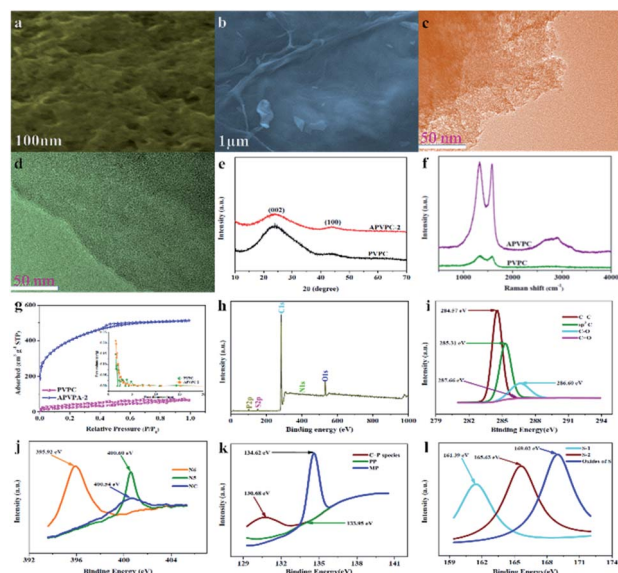
Fig. 1 (a) SEM images of APVPC-2. (b) SEM images of PVPC. (c) TEM images of APVPC-2. (d) TEM images of PVPC. (e) XRD patterns of PVPC and APVPC-2. (f) Raman spectra of PVPC and APVPC-2. (g) \text{N}_2 adsorption/desorption isotherms and the pore size distribution of APVPC-2 and PVPC. (h) XPS survey spectrum of APVPC-2. (i) High resolution C 1s spectrum of APVPC-2. (j) High resolution N 1s spectrum of APVPC-2. (k) High resolution P 2p spectrum of APVPC-2. (l) High resolution S 2p spectrum of APVPC-2.
