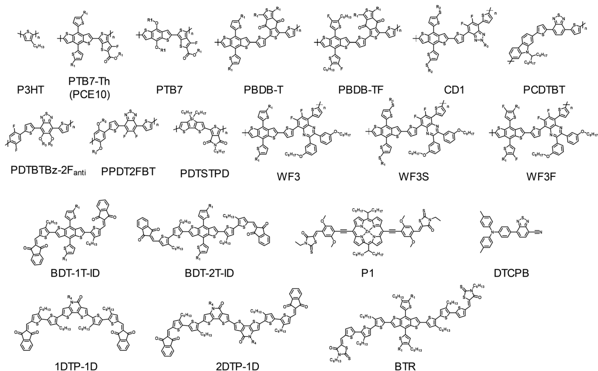
Fig. 3 Donor structures for indoor organic photovoltaic devices ( R_1 = 2-ethylhexyl, R_2 = 2-butyloctyl, R_3 = 2-hexyldecyl, R_4 = 2-octyldecyl, R_5 = 2-decyltetradecyl).
