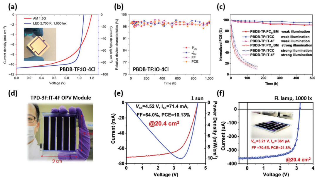
Fig. 8 Stable large-area indoor OPVs. (a) J - V characteristics of PBDB-TF:IO-4Cl devices (device area = 4 \text{ cm}^2 ) under 1 sun and LED illumination. (b) Stability results of photovoltaic parameters versus time. Reproduced from ref. 32 with permission from Springer Nature. (c) Device stability of PBDB-TF blends with PC 71 BM, ITCC and IT-4F under weak and strong illumination. Reproduced from ref. 63 with permission from WILEY-VCH. Indoor OPV modules. (d) Photograph of OPV modules. (e and f) J - V characteristics of TPD-3F:IT-4F-based OPV modules under AM 1.5G and FL lamp (1000 lx) illumination, respectively. Reproduced from ref. 64 with permission from Elsevier.
