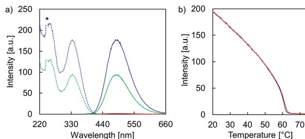
Fig. 5 (a) Fluorescence (solid line) and excitation (dotted line) spectra of A-B in aqueous medium at 75 ^{\circ} C (red), after thermally controlled assembly at 20 ^{\circ} C (blue), and at 20 ^{\circ} C after dialysis (green, <0.5 vol% ethanol). (b) Fluorescence-monitored annealing (blue) and melting (red) curves of A-B. Conditions: 1 \mu M A-B, 10 mM sodium phosphate buffer pH 7.2, 0.1 mM spermine-4 HCl, ethanol: 20 vol% (unless indicated otherwise), \lambda_{ex} : 335 nm, \lambda_{em} : 490 nm, temperature gradient: 0.5 ^{\circ} C min -1 , * indicates a second-order diffraction.
