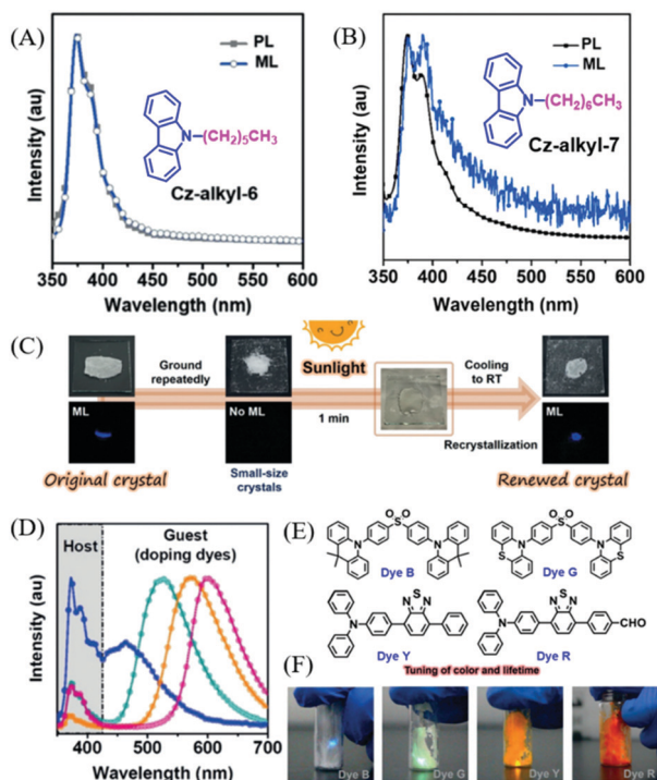
Fig. 6 (A) PL and ML spectra of Cz-alkyl-6 (A) and Cz-alkyl-7 (B); the inset shows the molecular structure. (C) The contactless solar-renewal process of Cz-alkyl-6 crystals by sunlight irradiation from a solar simulator. (D) ML spectra of Cz-alkyl-6 doping systems doped with dye B, dye G, dye Y, and dye R (from left to right). (E) The molecular structure of dyes B, G, Y and R. (F) ML photos of the doping system in daylight. Reproduced with permission. 59 Copyright 2018, John Wiley and Sons.
