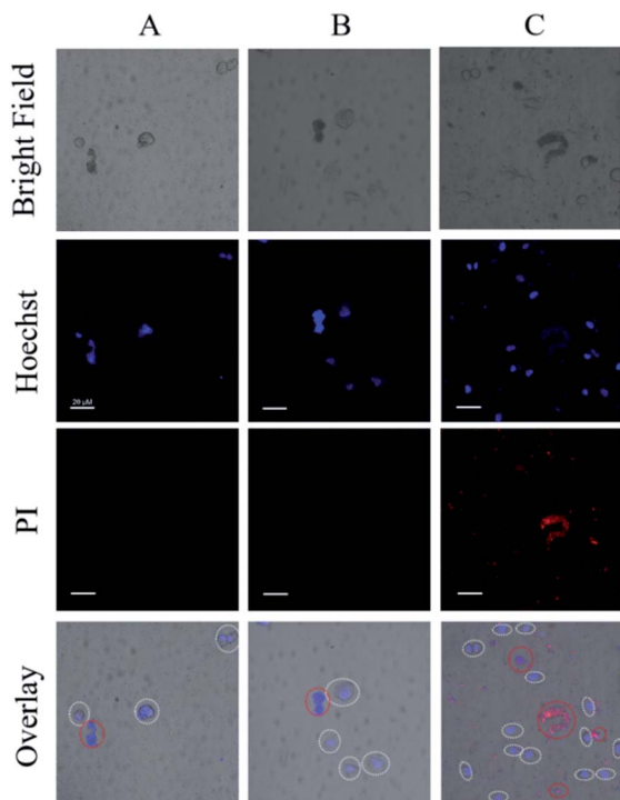
Fig. 7 CLSM images of the mixed solutions of S. aureus and L-O 2 . (A) light irradiation only, (B) addition of 4 (5 \mu\text{M} ) only, (C) addition of 4 (5 \mu\text{M} ) and light irradiation. For clarity, the L-O 2 cells were marked with white circles, red circles indicated the aggregated S. aureus cells (Scale bar: 20 \mu\text{m} ).
