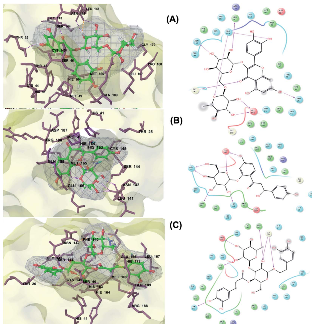
Fig. 1 3D (to the left) and 2D (to the right) interaction diagrams of (A) rutin, (B) rocymsosin b and (C) verbascoside with the crystal structure of 3CLpro (PDB ID: 5R7Y).
