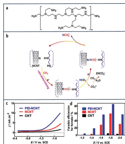
Fig. 12 (a) Structure of branched polyethylenimine (PEI). (b) Proposed mechanism for CO 2 reduction at PEI Functionalized, nitrogen-doped carbon nanotubes. (c) cathodic linear sweep voltammetry scans at 50 mV s -1 in a CO 2 -saturated aqueous 0.1 M KHCO 3 solution. (d) Plot of faradaic efficiencies for formate production vs. applied potential at CNT/GC, NCNT/GC, and PEI-NCNT/GC electrodes. 153 Copyright (2014) American Chemical Society.
