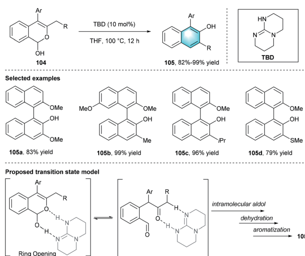
Scheme 29 TBD-catalyzed intramolecular benzannulation to synthesize substituted biaryls.
