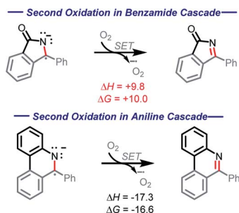
Scheme 13 Contrasting thermodynamics (kcal mol -1 ) for the C=N forming oxidations in the amide and aniline cascades.
