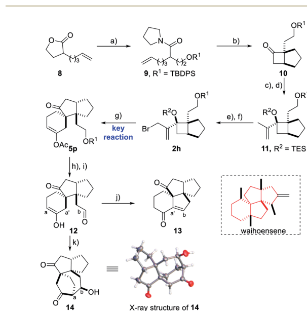
Scheme 3 Synthetic utility of the tetracyclic skeleton of waihoensene. Reagents and conditions: (a) pyrrolidine, Et 3 N, neat, 85 °C, then TBDPSCl, imidazole, CH 2 Cl 2 , 0 °C (98%); (b) Tf 2 O, 2,6-di- tert -butyl-4-methylpyridine, DCE, reflux, then CCl 4 /H 2 O reflux (54%); (c) 2-bromopropene, t -BuLi, THF, −78 °C (85% brsm); (d) TESOTf, 2,6-lutidine, CH 2 Cl 2 , 0 °C (94%); (e) SeO 2 , TBHP, CH 2 Cl 2 , 0 °C – rt (73% brsm); (f) CBr 4 , PPh 3 , imidazole, CH 2 Cl 2 , rt (90%); (g) prop-2-yn-1-yl acetate, CuOAc, Cs 2 CO 3 , DCE, 70 °C, then AuCl 3 , PTS, HFB (hexafluorobenzene), rt (40%, dr = 3.2 : 1); (h) TBAF, THF, 0 °C (93%); (i) IBX, EtOAc, reflux (91%); (j) K 2 CO 3 , MeOH/H 2 O = 100 : 1, 0 °C – rt (64%); (k) HCl, THF, rt (89%). TBDPSCl = tert -butyl diphenylchlorosilane, DCE = 1,2-dichloroethane, TESOTf = triethylsilyl tri-fluoromethanesulphonate, IBX = 2-iodoxybenzoic acid.
