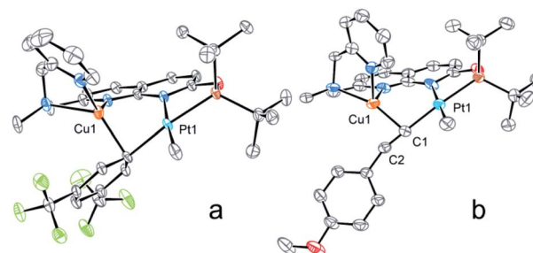
Fig. 4 ORTEP of 6 [B(Ar F ) 4 ] - (a) and 7 [BF 4 ] - (b) at the 50% probability level. Hydrogen atoms, counterions, and solvent molecules together with the minor disorder component for 7 [BF 4 ] - are omitted for clarity.
