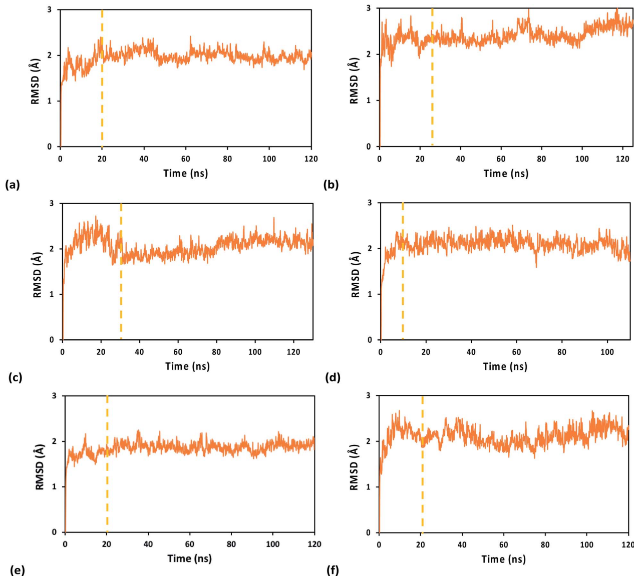
Fig. 2 RMSDs along the MD production runs for the WT (left) and Y345C (right) [Fe_4S_4] cluster-containing p58c protein from human primosome in complex with an RNA/DNA duplex. The MD simulations were carried out using the (a and b) A_{3+} , (c and d) 3_{3+} , and (e and f) A_{2+} FFs. The vertical dashed lines mark the start of the time window from which we extracted the system snapshots for the analysis of binding free energies and charge hopping pathways. The first snapshot in the MD run was used as the reference structure.
