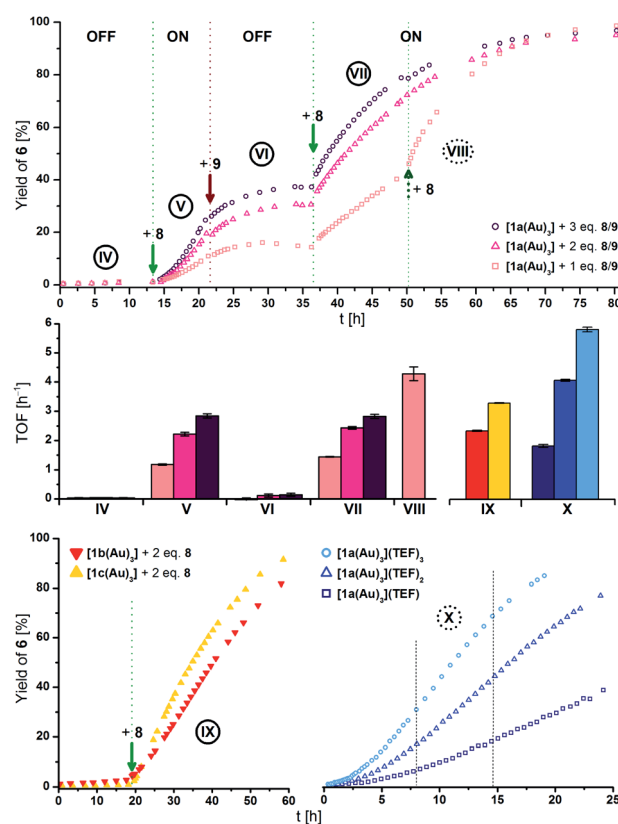
Fig. 5 (Top) Yield-over-time graphs for redox-switchable gold(i)-catalysed cyclisation of 5 to 6 using [1a(Au)_3] (1 mol% Au, [5]_0 = 60 mmol L^{-1} , CD_2Cl_2 , 25^\circ C ). Arrows indicate the addition of additives. IV: initial OFF phase; V: 1 st ON phase after addition of 1.0–3.0 eq. oxidant 8 ; VI: 2 nd OFF phase after addition of 1.1–3.3 eq. reductant 9 ; VII: 2 nd ON phase after addition of 1.1–3.3 eq. oxidant 8 ; VIII: addition of 2.2 eq. 8 to 1 eq.-switched reaction (rose squares). (Centre) Comparison of turn-over frequencies (TOF) determined from linear fits (cf. Fig. S40–S48† for regression plots) of reaction phases IV to VIII (top), IX (bottom left), and X (bottom right). (Bottom) Left: yield-over-time graphs for gold(i)-catalysed cyclisation of 5 to 6 using [1b(Au)_3] (red) and [1c(Au)_3] (yellow; conditions as above), oxidised in situ with 2 eq. of 8 . Right: yield-over-time graphs for gold(i)-catalysed cyclisation of 5 to 6 using isolated oxidised complexes [1a(Au)_3](TEF)_n ( n = 1–3 , conditions as above). Dashed lines represent the chosen timeframe for linear fitting.
