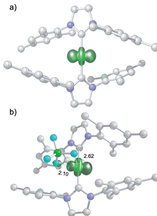
Fig. 5 (a) Spin density plot for [\text{Ni}(\text{Mes}_2\text{Im})_2]^+ ; (b) molecular structure of \mathbf{8}_{\text{DFT}}^1 showing \text{Ni}-\text{F}^{\text{BF}_4^-} contacts (isovalue \pm 0.0075\text{ a}_0^{-3} ; lengths of \text{Ni}-\text{F} contacts in \text{\AA} ; hydrogen atoms not shown).
