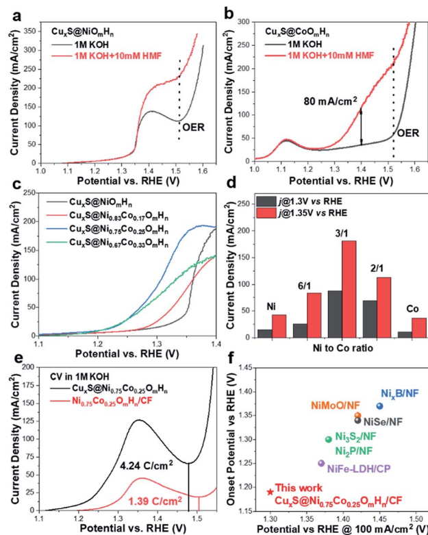
Fig. 2 (a and b) LSV curves of \text{Cu}_x\text{S}@\text{NiO}_m\text{H}_n and \text{Cu}_x\text{S}@\text{CoO}_m\text{H}_n towards electrochemical HMF oxidation. (c) Comparison of LSV curves of \text{Cu}_x\text{S}@\text{NiCo} LDHs with various Ni to Co ratios. (d) Current densities of prepared electrodes at 1.3 V and 1.35 V vs. RHE. (e) CV curves of \text{Cu}_x\text{S}@\text{Ni}_{0.75}\text{Co}_{0.25}\text{O}_m\text{H}_n , \text{Ni}_{0.75}\text{Co}_{0.25}\text{O}_m\text{H}_n/\text{CF} in 1 M KOH and calculated charges for the oxidation of transition metal cations prior to the oxygen evolution reaction. (f) Performance comparison of \text{Cu}_x\text{S}@\text{Ni}_{0.75}\text{Co}_{0.25}\text{O}_m\text{H}_n/\text{CF} with reported electrocatalysts towards electrochemical oxidation of HMF, urea and primary amine.
