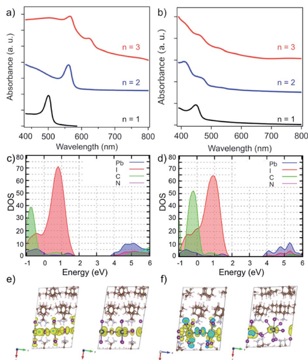
Fig. 5 Optoelectronic properties of perovskite thin films. UV-vis absorption spectra of perovskite thin films based on (a) A_2FA_{n-1}Pb_nI_{3n+1} and (b) A'_2FA_{n-1}Pb_nI_{3n+1} ( n = 1 – 3 ) compositions on FTO/mp-TiO 2 substrates in accordance with the previous report. 13 Calculated partial density of states for (c) A_2PbI_4 and (d) A'_2PbI_4 with (e and f) the corresponding frontier molecular orbitals (top of the valence band (left) and bottom of the conduction band (right)).
