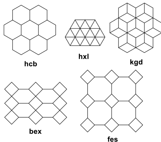
Chart 3 Most commonly occurring 2D topologies 29 for CTV-type coordination polymers.
