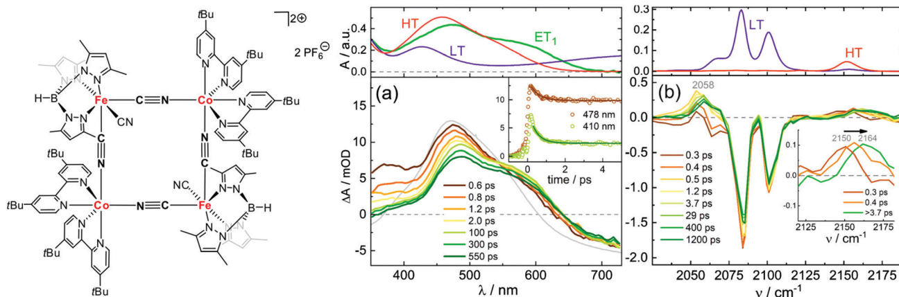
Fig. 2 Structure of [(\text{Co}_{\text{LS}}^{\text{II}})_2(\text{Fe}_{\text{LS}}^{\text{II}})_2] together with transient absorption data in acetonitrile at -30^\circ\text{C} with (a) UV-visible probe and 775 nm pump wavelength and (b) IR probe and 800 nm pump. The top panels show the static absorption spectra in the LT ( -30^\circ\text{C} ) and HT ( 30^\circ\text{C} ) phases. The green line (ET1) corresponds to the calculated spectrum of the one-electron transfer product [\text{Co}_{\text{LS}}^{\text{III}}\text{Fe}_{\text{LS}}^{\text{II}}\text{Co}_{\text{HS}}^{\text{I}}\text{Fe}_{\text{LS}}^{\text{II}}] . The bottom panels show the time-resolved spectra at selected time delays. The grey line shows the difference between the HT and LT static spectra. Reprinted with permission from Zimara et al. Inorganic Chemistry, 2021, 60 , 449–459. 116 Copyright 2021 American Chemical Society.
