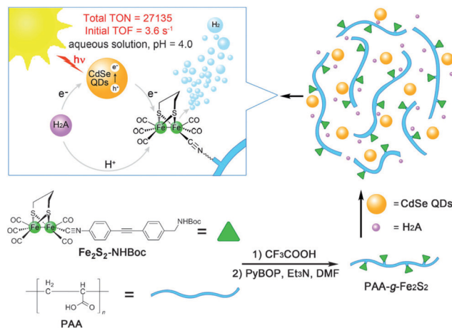
Fig. 115 Synthetic pathway towards modified pdt and representation of photocatalytic activity. Reprinted from ref. 165 with permission from John Wiley and Sons, Copyright 2013.
