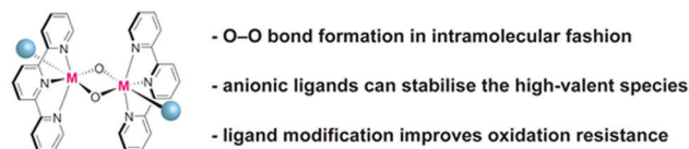
Chart 13 Summary of features of water oxidation catalysts with dimeric structures.
