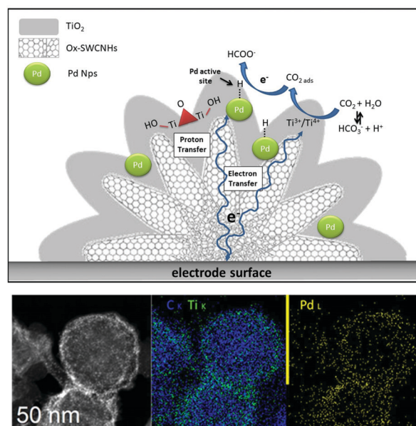
Fig. 6 Top: Graphical sketch of the PdNP/ \text{TiO}_2\text{@CNH} nanostructure and of the interfacial synergy towards the reversible \text{HCOOH} formation; bottom: HAAFD (black and white) and EDX elemental mapping of C, Ti and Pd confirming the co-location of the three elements.
