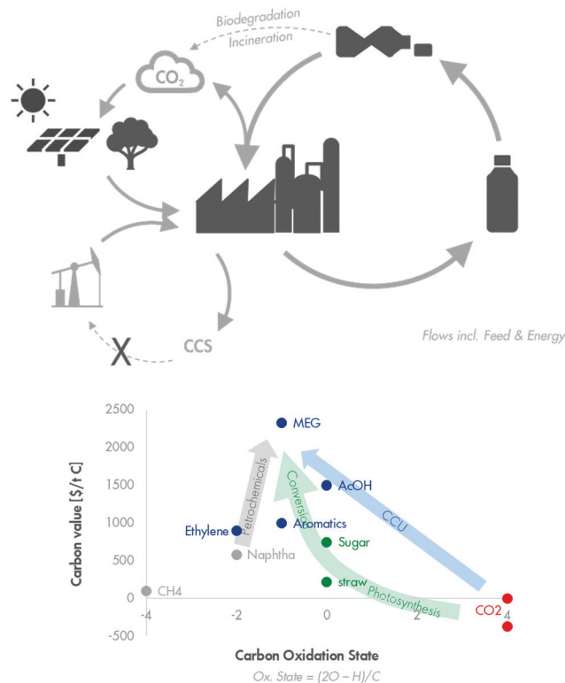
Fig. 8 Artist's impression of future sustainable carbon-chemical cycles (top) and shift in feedstock oxidation state (bottom); the carbon value has been defined as market price divided by carbon content, the carbon oxidation state has been calculated from the C : H : O ratio of the product following the eq. reported in the figure).
