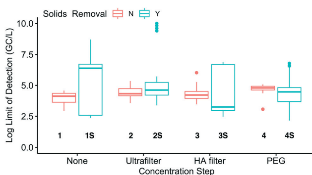
Fig. 6 Comparison of the log-transformed theoretical limits of detection (combined for Plant 1 and Plant 2) for each of the eight method groups (grouped by concentration step and solids removal).
