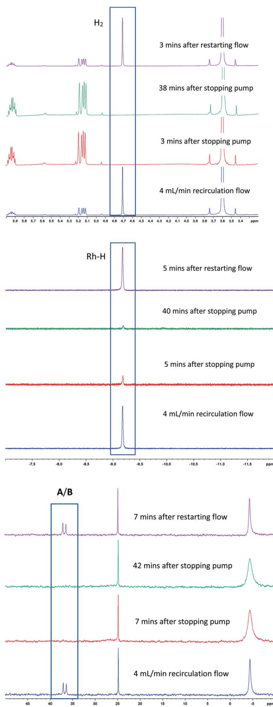
Fig. 13 1 H and 31 P{ 1 H} FlowNMR spectra of [Rh(CO) 2 (acac)] + 6PPh 3 catalysed hydroformylation of 1-hexene in toluene at 50 °C and 12 bar of H 2 /CO (1 : 1) during stop/start cycling of flow. [Rh(CO) 2 (acac)] = 2.5 mM, [1-hexene] = 500 mM, [PPh 3 ] = 15 mM.
