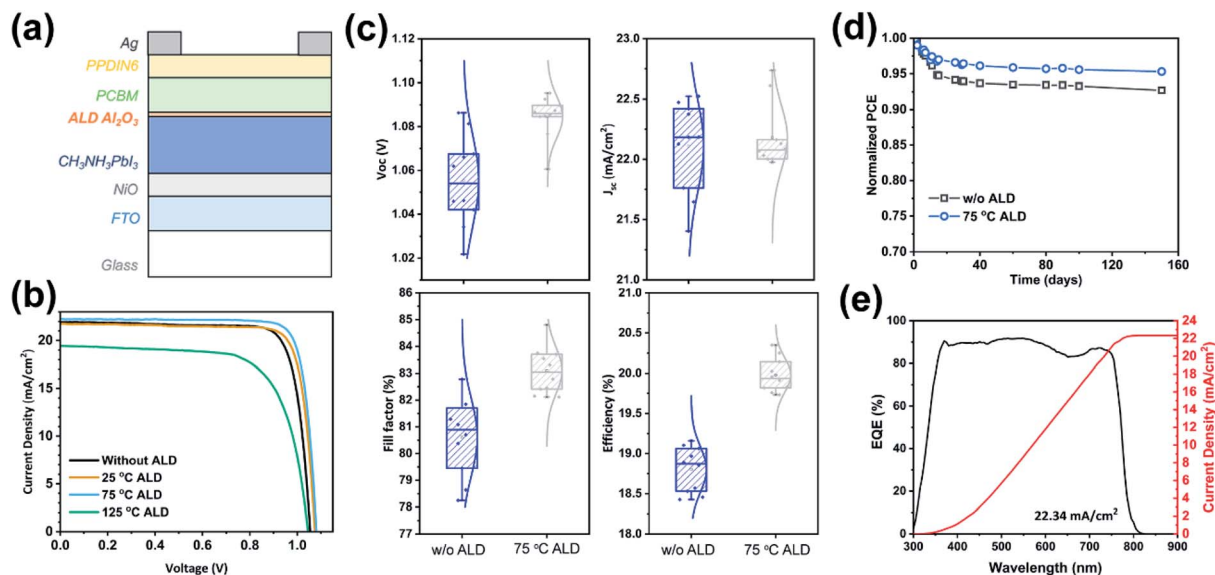
Fig. 3 (a) Schematic architecture of the ambient-prepared PSCs with an ALD \text{Al}_2\text{O}_3 interlayer: FTO/ \text{NiO}_x /MAPbI 3 /ALD- \text{Al}_2\text{O}_3 /PCBM/PPDI 6 /Ag. (b) Curves of current density versus voltage ( J - V ) for the PSCs with and without 10 cycles of ALD of \text{Al}_2\text{O}_3 deposited at 25 °C, 75 °C and 125 °C, and the corresponding statistical distributions of performance parameters are shown in Fig. S2† (c) Statistical distributions of V_{\text{oc}} , J_{\text{sc}} , fill factor, and PCE for the PSCs with and without ALD \text{Al}_2\text{O}_3 deposited at 75 °C. (d) Long-term stability of PSCs in a \text{N}_2 atmosphere. (e) Incident photon-to-electron conversion efficiency (IPCE) spectrum and the corresponding integrated current density for the PSCs with 10 cycles of ALD of \text{Al}_2\text{O}_3 at 75 °C ((b): 75 °C ALD).
