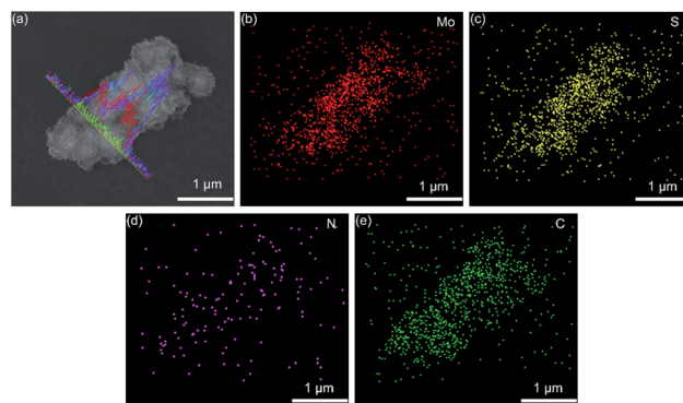
Fig. 3 (a) SEM and (b–e) elemental mapping images of MoS 2 @C@PANI. Line-scan profiles are inserted in (a).
