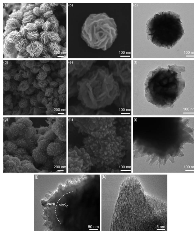
Fig. 2 SEM images of (a and b) flower-shaped MoS 2 , (d and e) MoS 2 @C, and (g and h) MoS 2 @C@PANI. TEM images of the (c) bare MoS 2 , (f) MoS 2 @C composite and (i) MoS 2 @C@PANI. (j and k) HRTEM images of MoS 2 @C@PANI. The dashed line in j indicates the boundary between MoS 2 and PANI.
