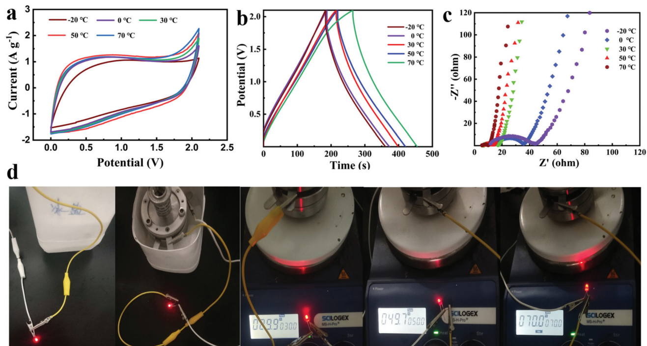
Fig. 5 The NG//NG quasi-solid-state supercapacitor with the PAAK/CMC-24 M polyelectrolyte hydrogel working at different temperatures: CV curves at 10 \text{ mV s}^{-1} (a), GCD curves at 0.5 \text{ A g}^{-1} (b), EIS (c), LED powered (d).
