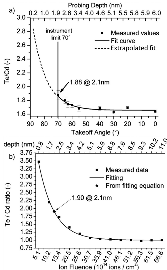
Fig. 11 (a) Te: Cd ratio from a sequence of ARXPS measurements compared with (b) a profile of sequential 5 keV Ne + ISS measurements as a comparison probe of the two methods efficacy in the analysis of ultra-thin films. 216
