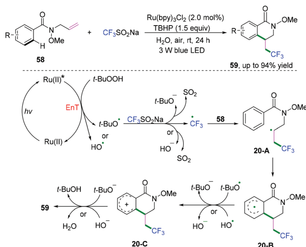
Scheme 32 Visible-light-induced radical cyclization of N -allylbenzamides with CF 3 SO 2 Na.
